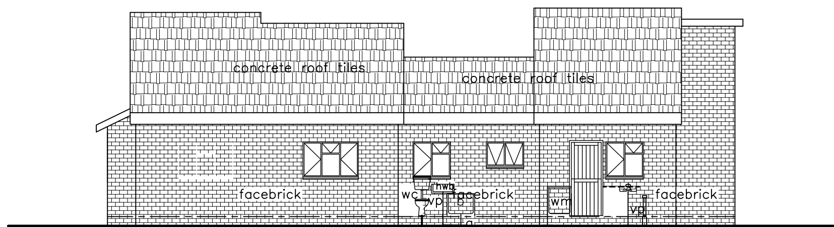
BACK / WESTERN ELEVATION Scale 1:100
