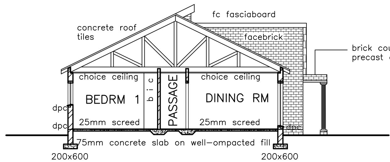
SECTION C-C Scale 1:100
