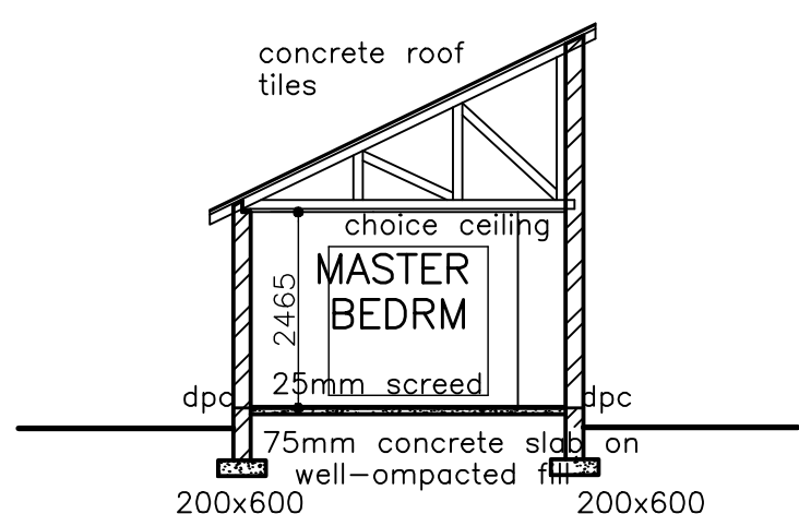
SECTION D-D Scale 1:100
