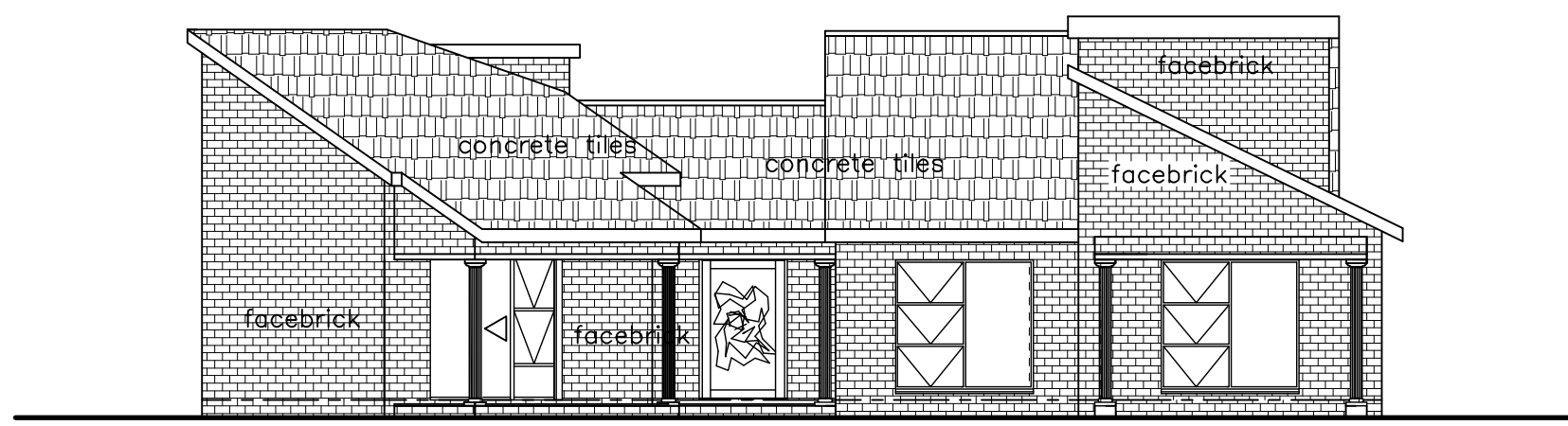
FRONT / EASTERN ELEVATION Scale 1:100
