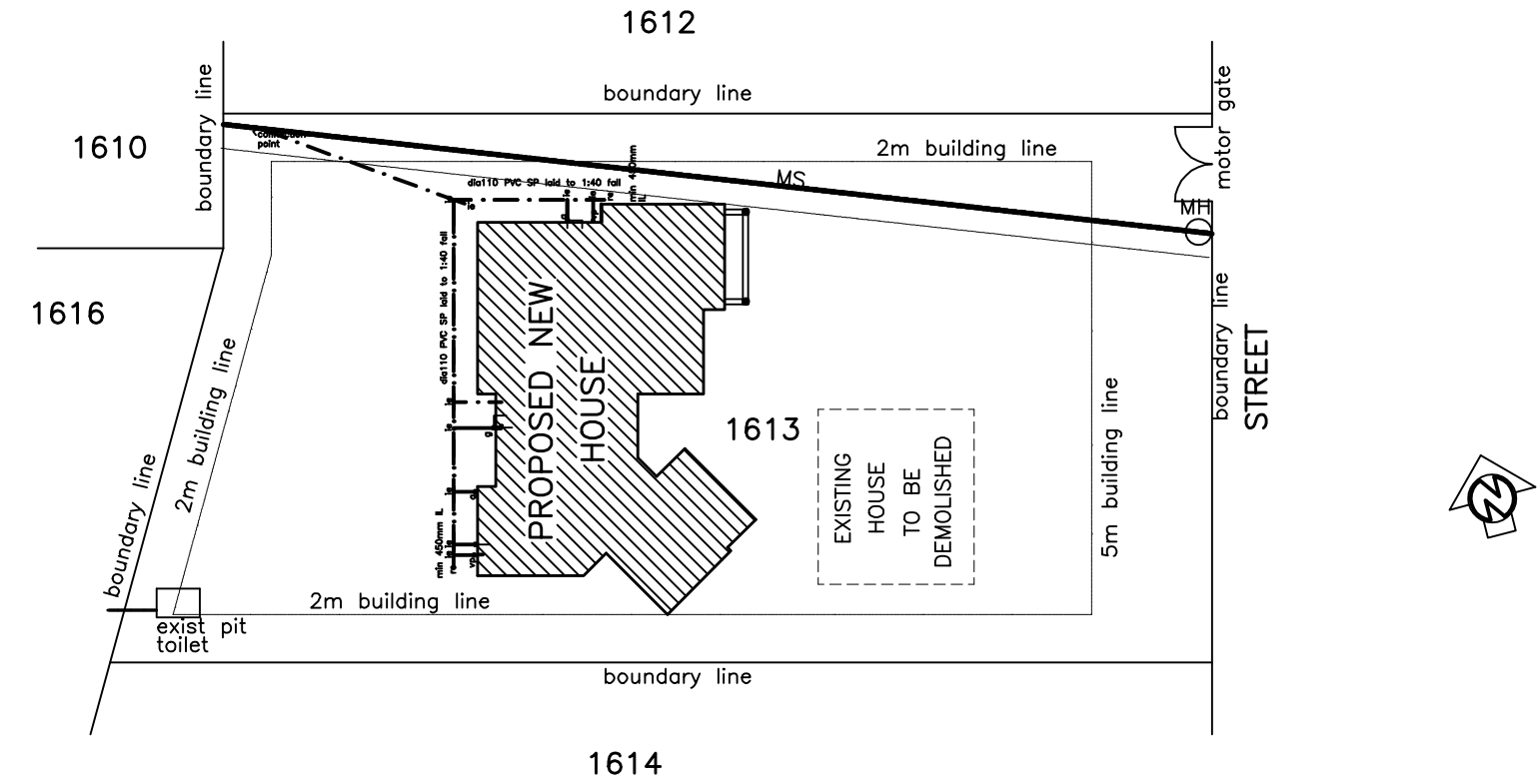
SITE PLAN Scale 1:300
